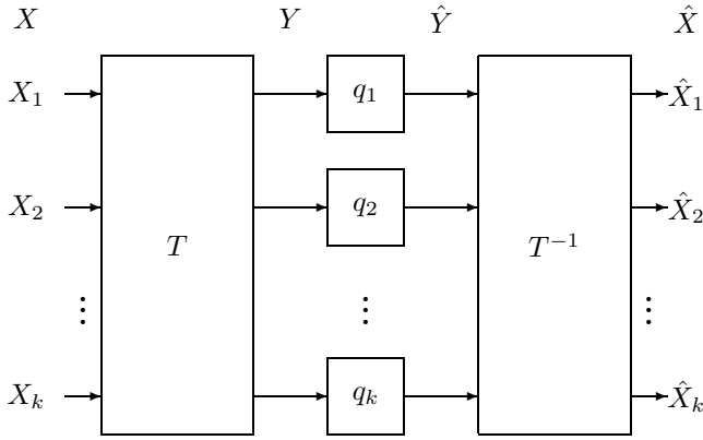
Fig. 4. Transform Code
