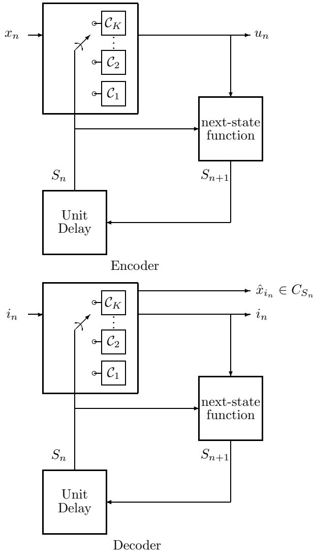
Fig. 10. Finite-state vector quantizer
