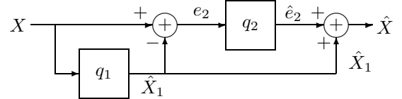
Fig. 9. Two-Stage VQ
