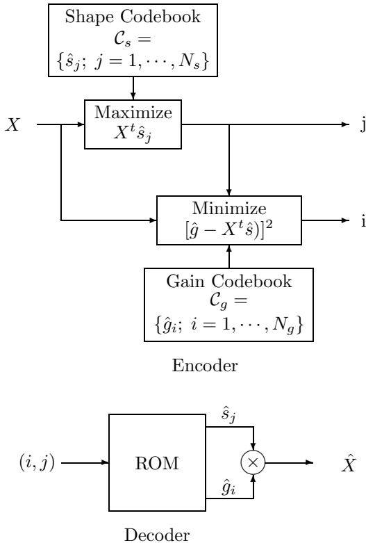
Fig. 8. Shape-Gain VQ
