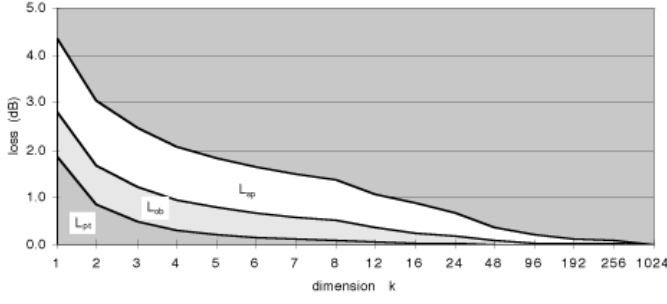
Fig. 5. Losses of optimal k -dimensional quantization relative to optimal high-dimensional quantization for an i.i.d. Gaussian source. The bottom curve is point density loss; above that is point density loss plus oblongity loss; and the top curve is the total loss. For k \geq 4 , the space filling losses are estimates.
