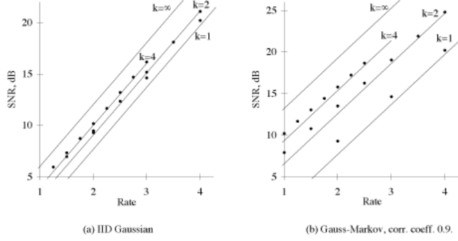
Fig. 7. Signal-to-noise ratios for optimal VQs (dots) and predictions thereof based on the Zador-Gersho formula (straight lines).
